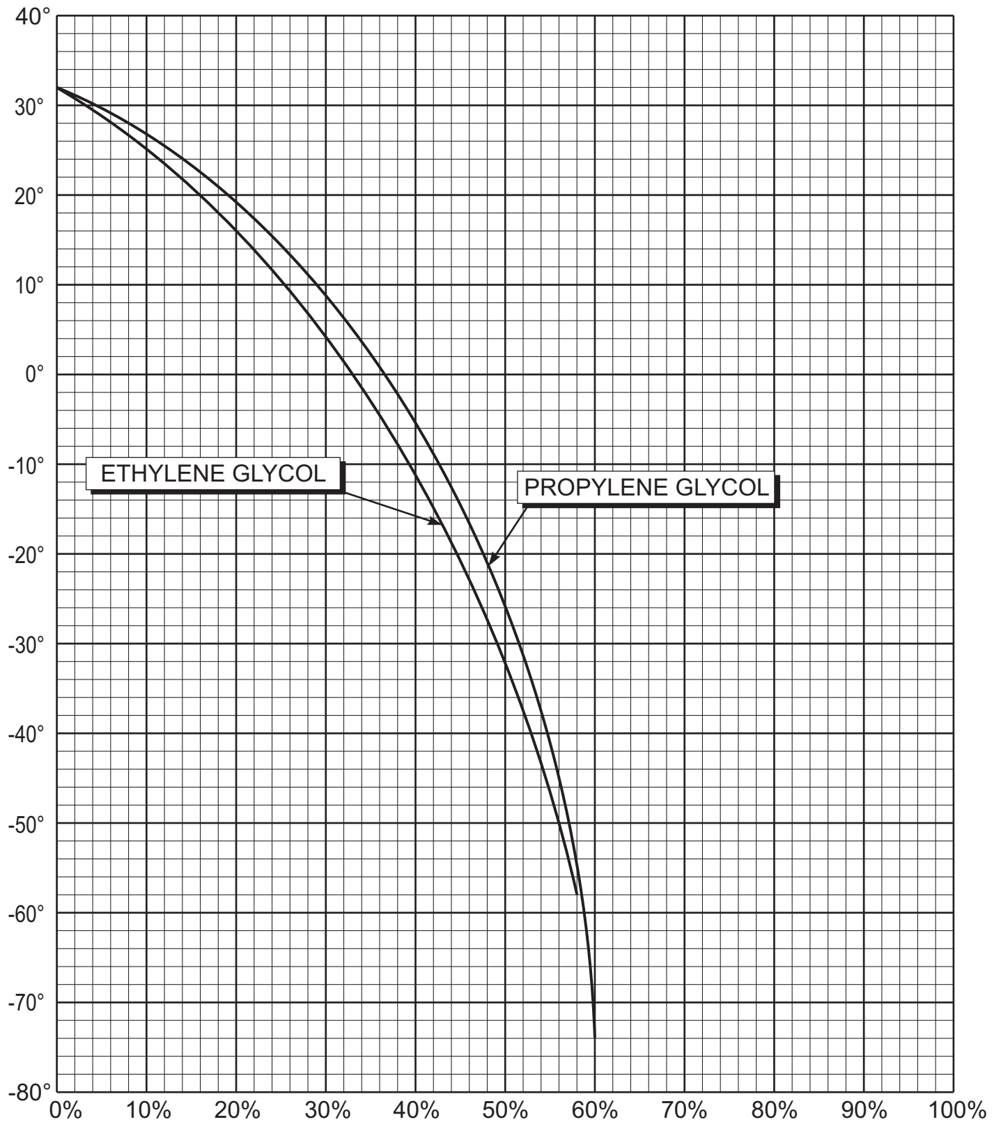
FREEZING POINT of WATER/GLYCOL SOLUTIONS
